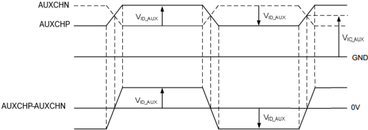
AUX CH V ID_AUX and V IC_AUX definition
