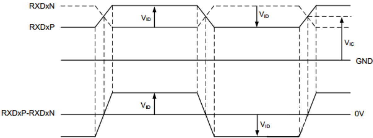
Main Link V ID and V IC definition
